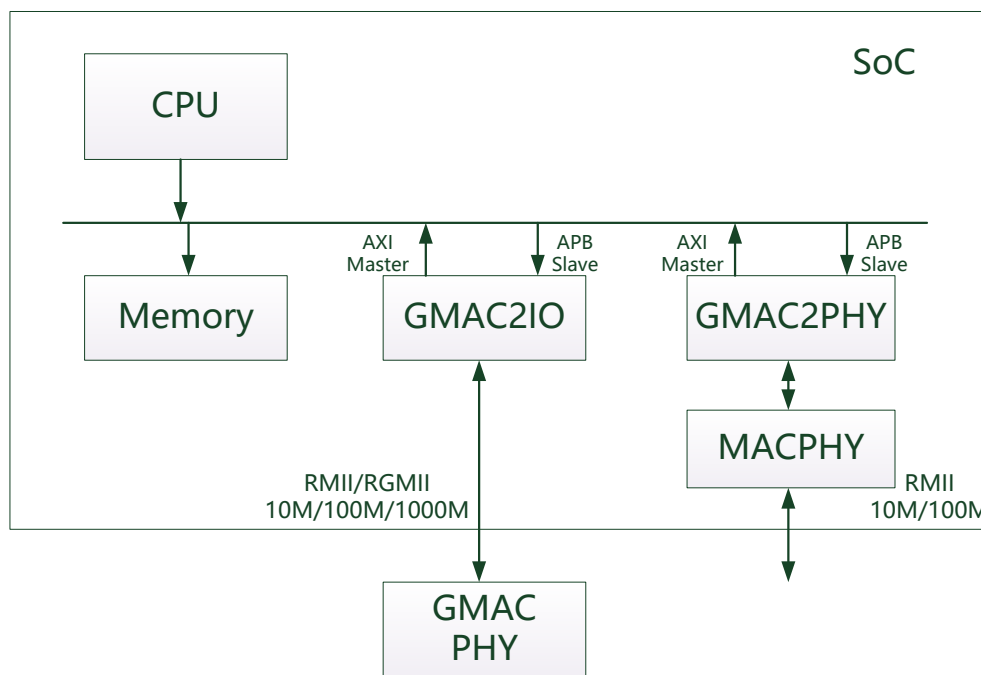
Fig.22-1 GMAC Architecture
