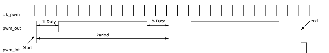
Fig. 16-5 PWM One-shot Center-aligned Output Mode
