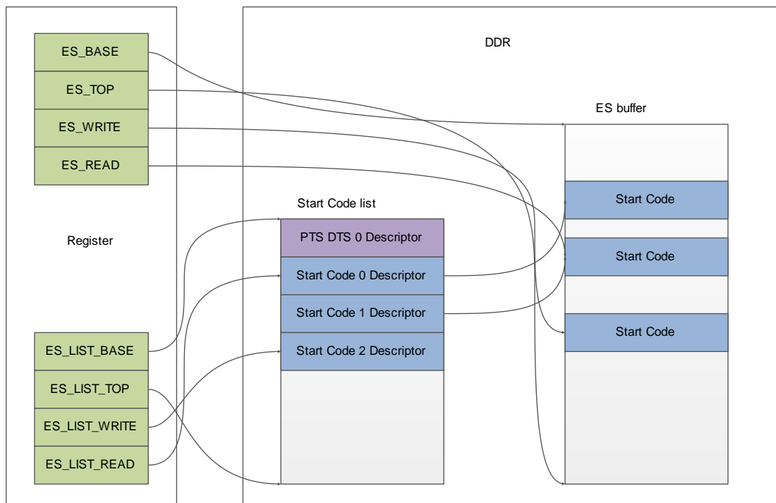
Fig. 1-7LLPmemory architecture
