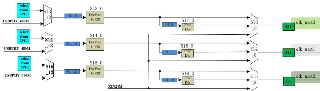
Fig. 17-10 UART clock generation
