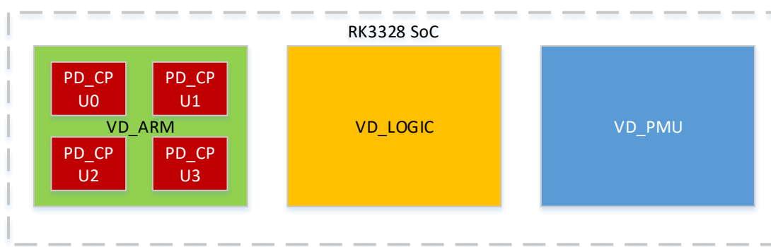
Fig. 6-1 RK3328 Power Domain Partition
