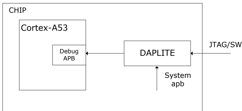
Fig. 11-1 Debug system structure
