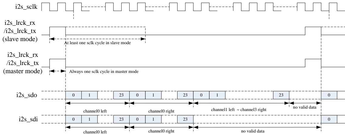
Fig. 25-8 PCM late1 mode timing format
