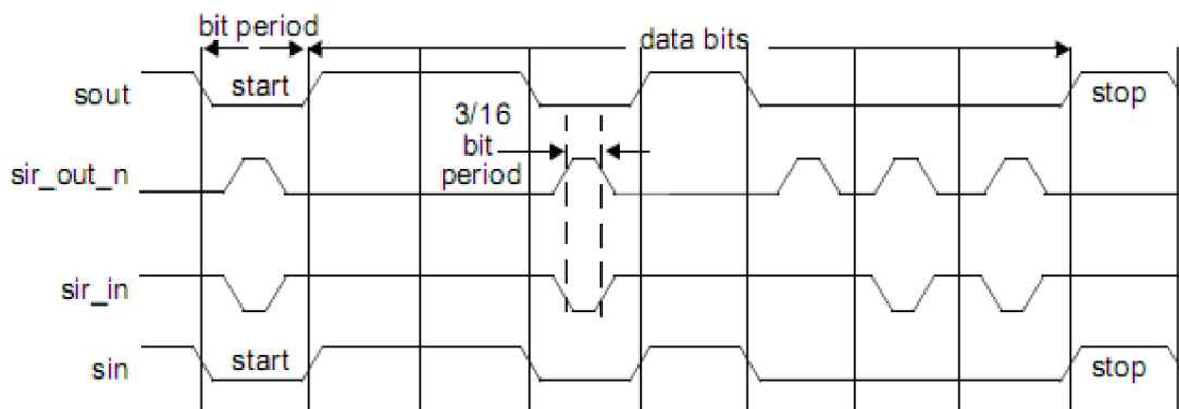
Fig. 17-3 IrDA 1.0
