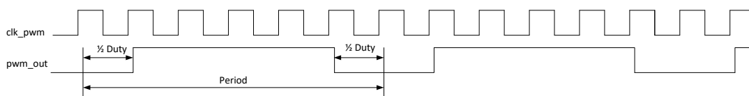
Fig. 16-4 PWM Continuous Center-aligned Output Mode
