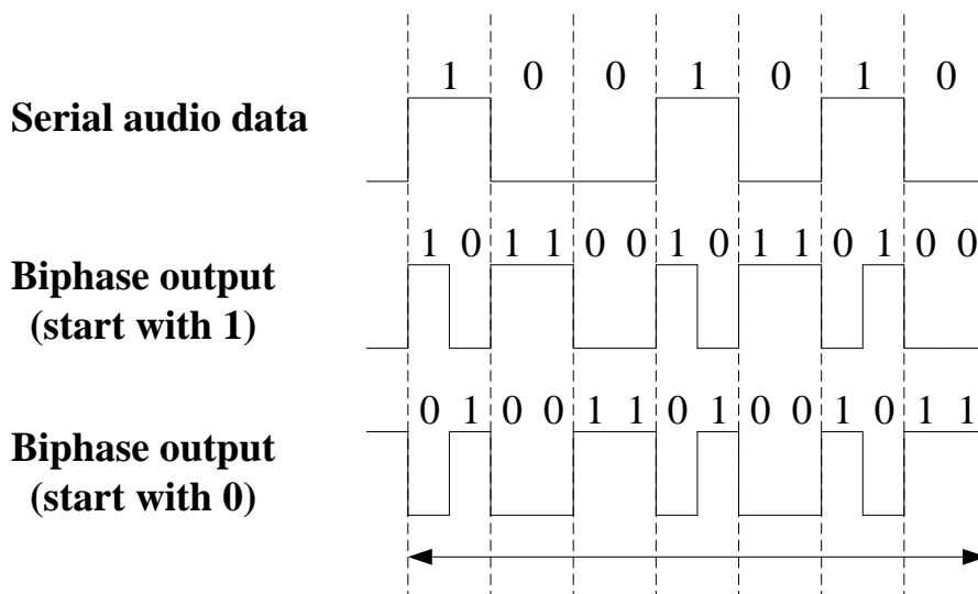
Fig.21-4 SPDIF Channel Coding
