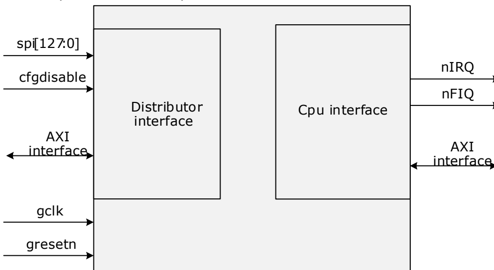
Fig. 7-1 Block Diagram
