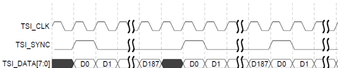
Fig. 15-4 Sync/Burst Parallel Mode
