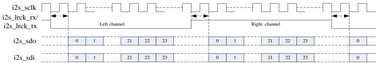
Fig. 25-4 I2S normal mode timing format
