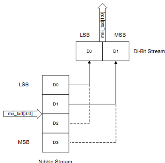
Fig.22-3 RMI transmission bit ordering
