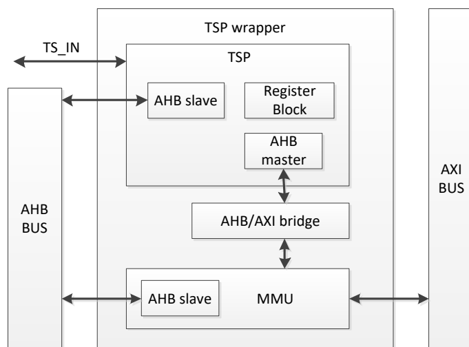
Fig. 15-1 TSP architecture
