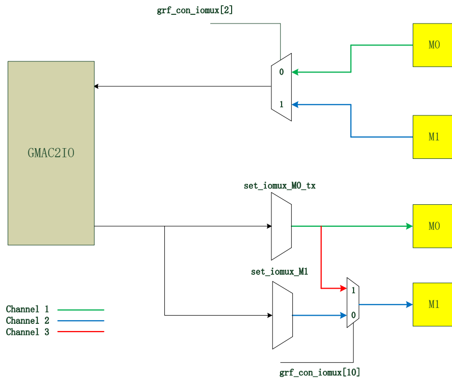
Fig. 22-16 gmac2io channel architecture
